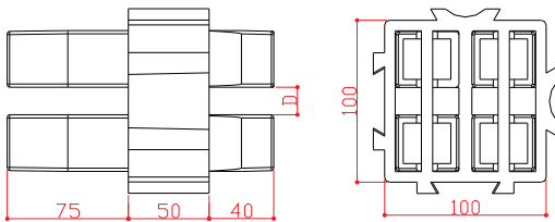
2. 棧板腳架 Foot plate connection
